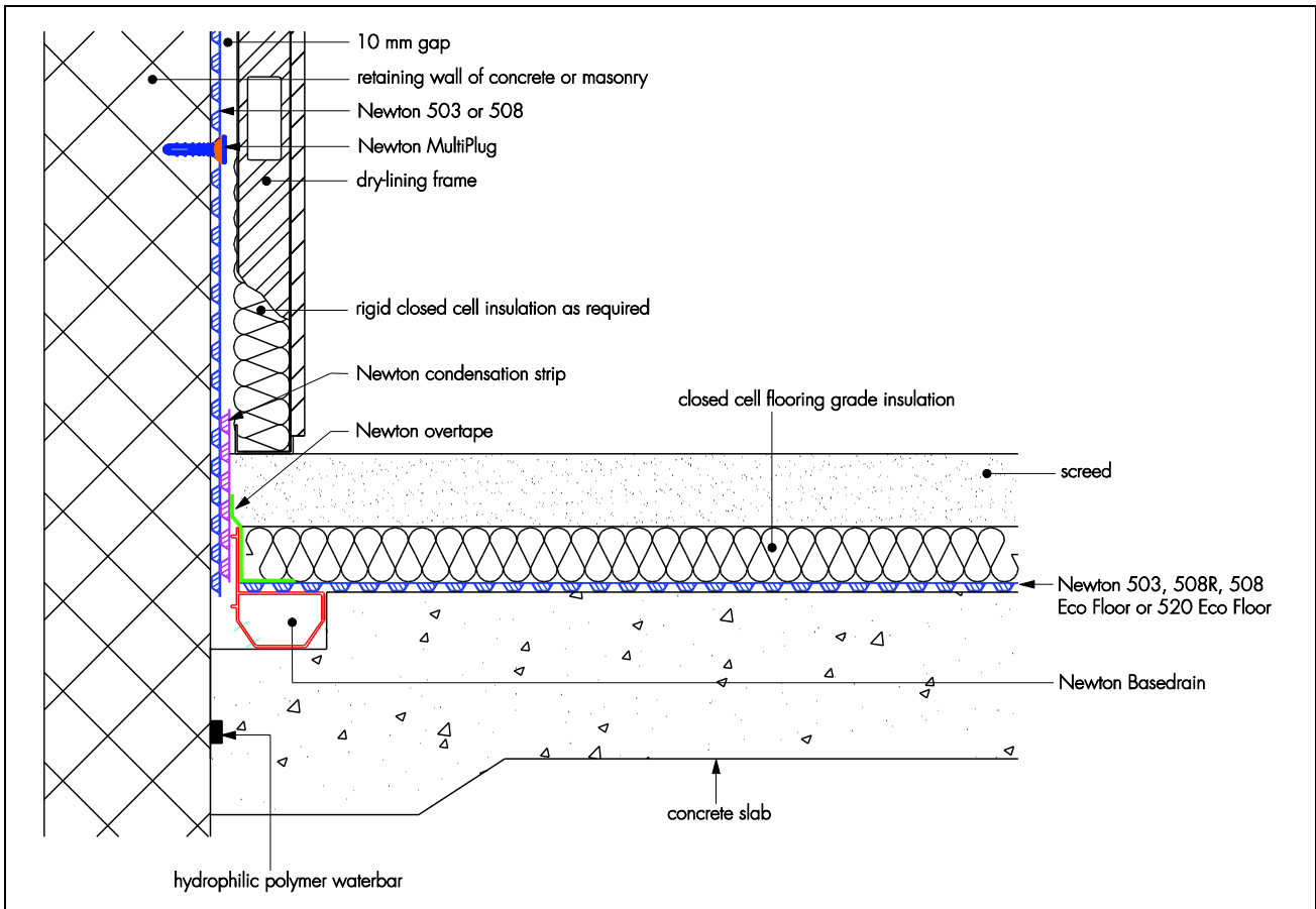
Figure 3 Installation detail
