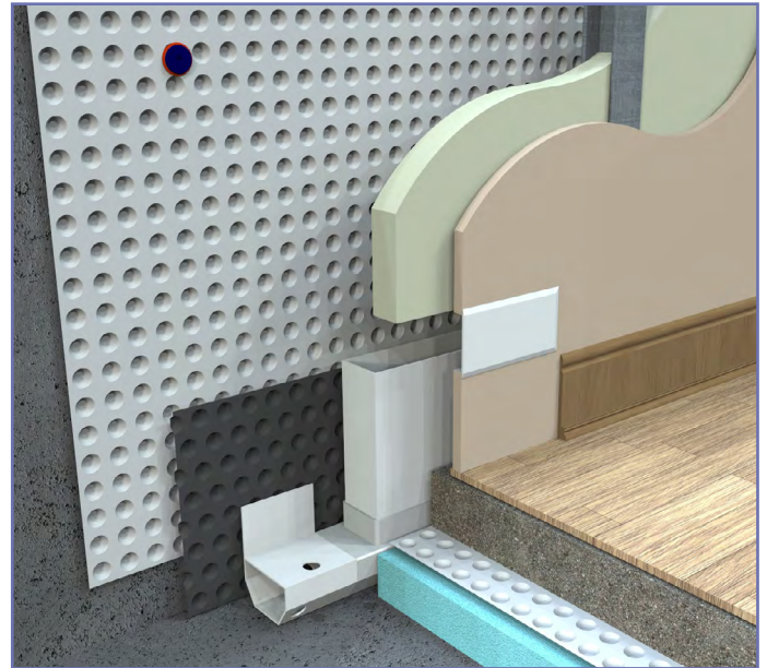
Figure 2: A Newton inspection port in a maintainable Type C system
